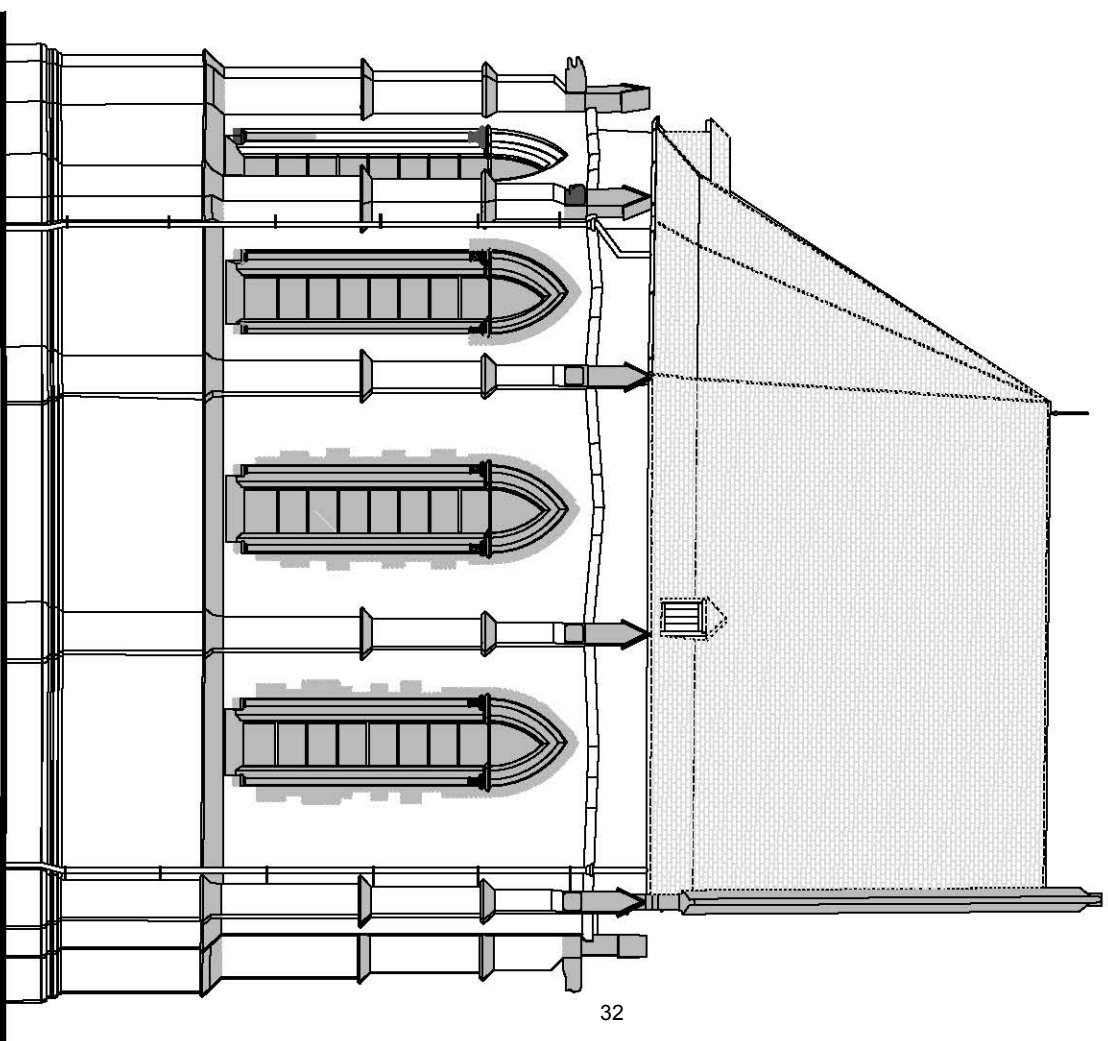
FACADE NORD - NOORDGEVEL
